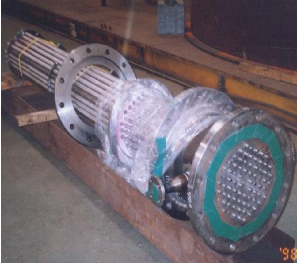
Heat Exchanger
